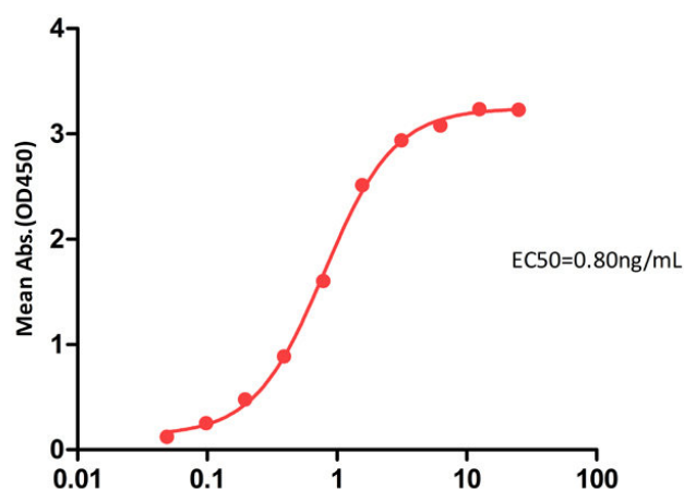
Anti-SARS-CoV-2 RBD Potent Neutralizing Antibody, Chimeric mAb, Human IgG1 (AM128) Conc.(ng/ml)
