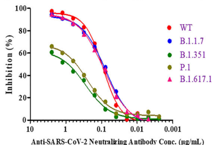
Inhibition of SARS-CoV-2 Spike RBD:ACE2 Interaction by Anti-SARS-CoV-2 Neutralizing Antibody (Cat.No. SPD-M128)
