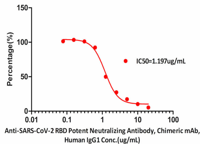
Anti-SARS-CoV-2 RBD Potent Neutralizing Antibody, Chimeric mAb, Human IgG1 (AM128)ELISA
