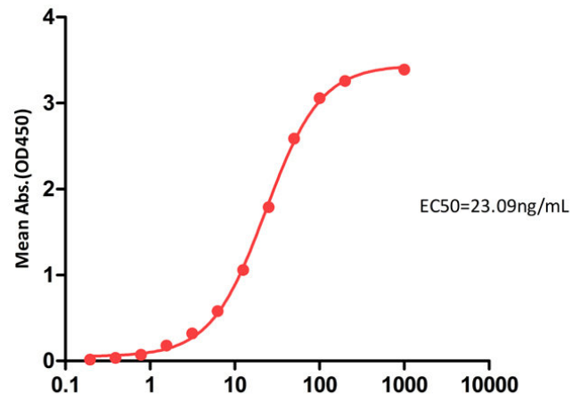
Biotinylated Anti-SARS-CoV-2 Spike RBD Antibody, Chimeric mAb, Human IgG1 (AM130) ELISA 0.2 μg of SARS-CoV-2 (COVID-19) S protein RBD, His Tag per well
