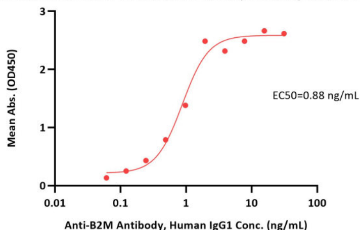
PE-Labeled Human HLA-A*02:01&B2M&HPV16-E6 (TIHDIILECV) Tetramer Protein ELISA 0.1 µg of PE-Labeled Human HLA-A*02:01&B2M&HPV16-E6 (TIHDIILECV) Tetramer Protein per well
