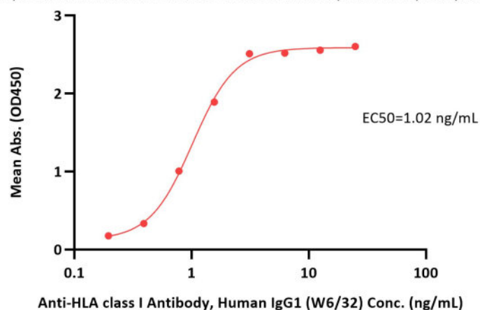
Biotinylated Human HLA-A*24:02&B2M&EBV EBNA3A (RYSIFFDYM) Complex Protein ELISA 0.1 µg of Biotinylated Human HLA-A*24:02&B2M&EBV EBNA3A (RYSIFFDYM) Complex Protein per well
