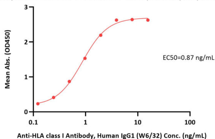
Biotinylated Human HLA-A*11:01&B2M&HPV16-E7 (IVCPICSQK) Complex Protein ELISA 0.1 µg of Biotinylated Human HLA-A*11:01&B2M&HPV16-E7 (IVCPICSQK) Complex Protein per well
