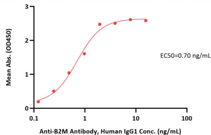
Biotinylated Human HLA-A*11:01&B2M&EBV LMP2 (SSCSSCPLSK) Complex Protein ELISA 0.1 µg of Biotinylated Human HLA-A*11:01&B2M&EBV LMP2 (SSCSSCPLSK) Complex Protein per well
