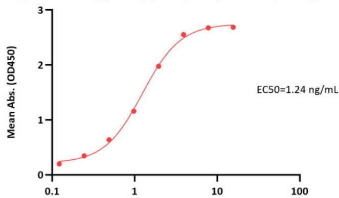
Monoclonal Anti-Influenza A [A/Darwin/9/2021 (H3N2)] HA Antibody, Human IgG1 (1D6) Conc. (ng/mL)
